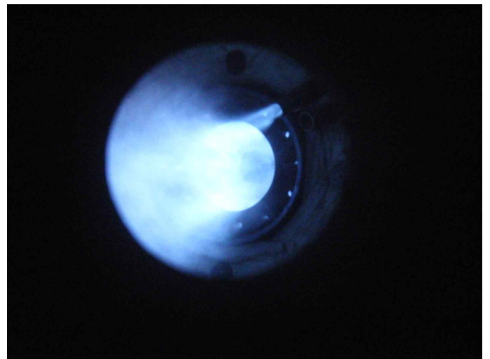
2-15. TMS-Rotary kiln \Phi 560 \times 6,000L 1,000°C
